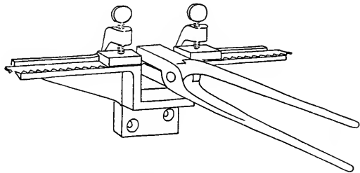
FIG. 188. BRAZING CLAMP FOR BAND-SAWS.
